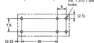
Mounting Holes (Bottom View)
